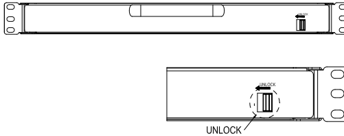
Figure 3-3 unlocking
